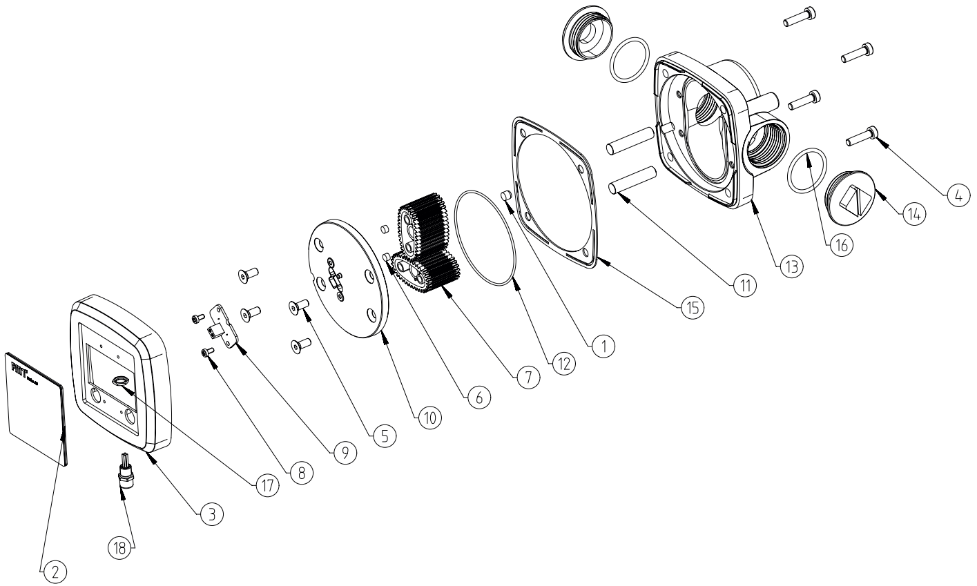
Fig. 15-1: Exploded view pulse meter and digital oval gear meter without display
