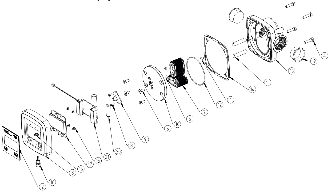
Fig. 16-1: Exploded view pulse meter and digital oval gear meter - with display
